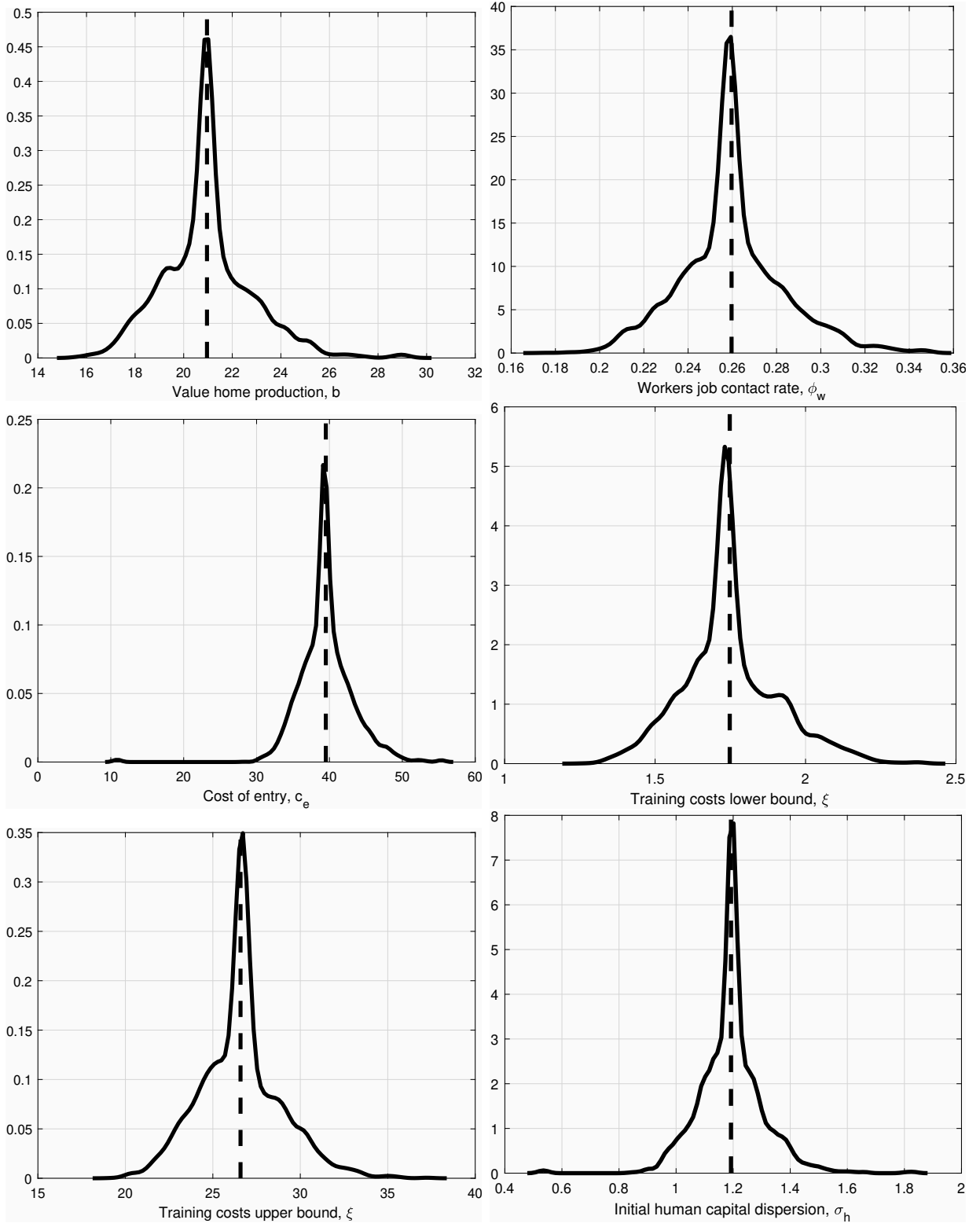
Figure 11: Posterior distributions
